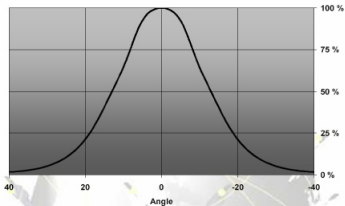
Relative Luminous Intensity (%)
